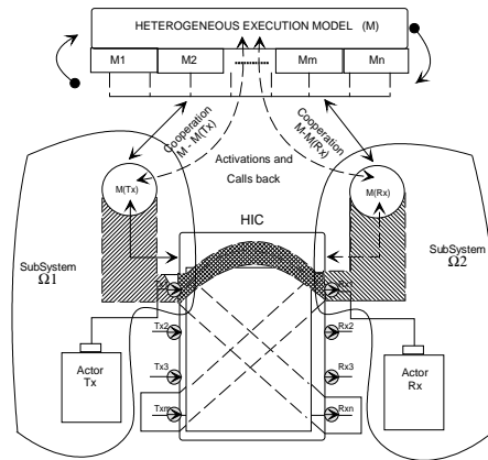
Figure 3. HIC - Execution Model Cooperation
