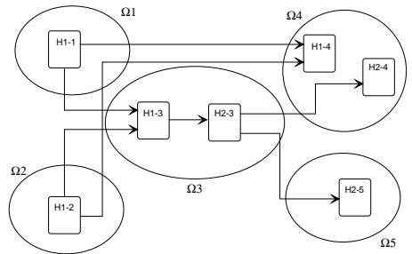
Figure 12. Skeleton of the example system
