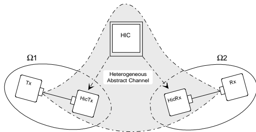
Figure 4. Heterogeneous abstract channel
