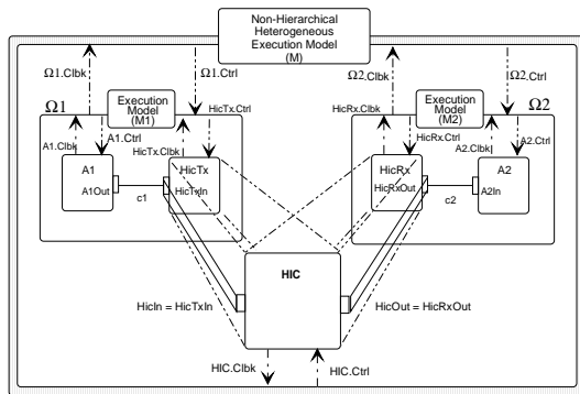
Figure 2. A HIC projected on two domains
